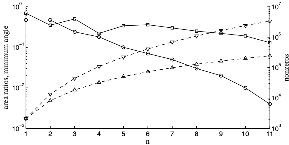
FIG. 2.4. Mesh diagnostics: The number of connections in both A_s (▽) and in A_f (△) along with the normalized minimum angle (□) and the area ratio (○) in the finite element mesh.
