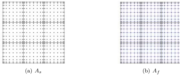
FIG. 1.2. Meshes corresponding to the spectral element operator A_s and to the finite element preconditioner A_f , respectively.
