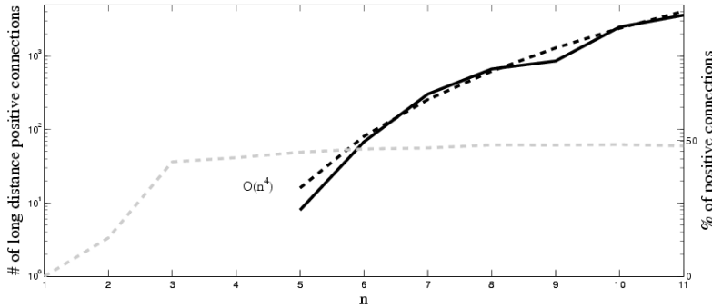
FIG. 2.6. The increase in positive off-diagonal connections that do not have a sufficiently large negatively weighted path of length two (solid line). The dark dashed line is the \mathcal{O}(n^4) reference, and the dashed gray line indicates the percentage of off-diagonals that are positive.
