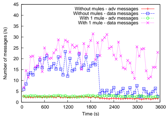
Fig. 13. Comparison of number of messages per second at different time
