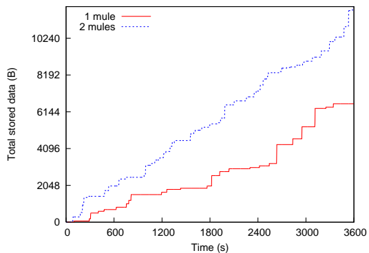
Fig. 15. Total stored data of the basestation over time
