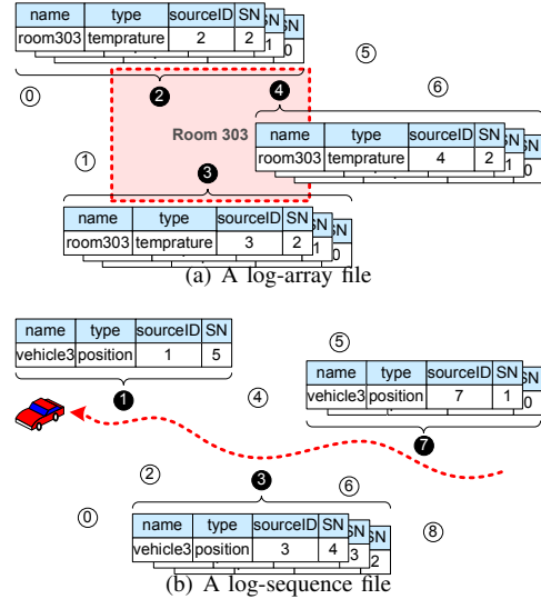
Fig. 5. Examples of different types of log files
