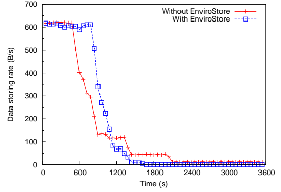
Fig. 10. Data storing rate at different time
