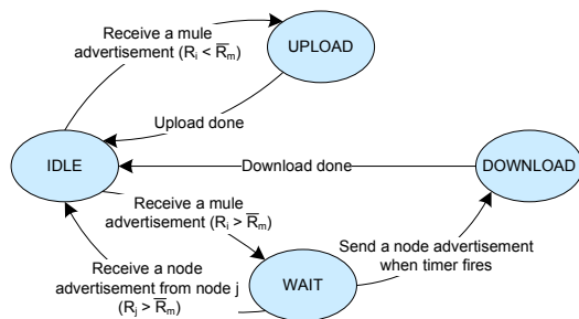
Fig. 2. State transition of a sensor node in cross-partition data redistribution
