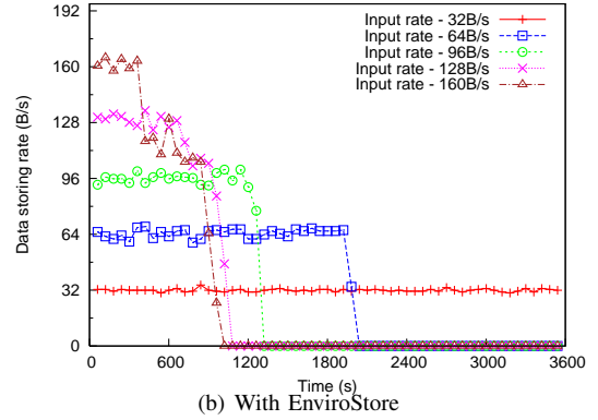
Fig. 7. Data storing rate at different time
