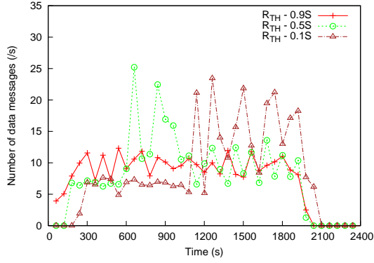
Fig. 8. Comparison of data storing rate at different time
