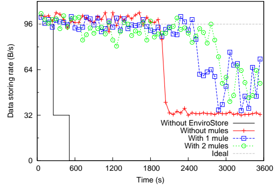
Fig. 11. Comparison of data storing rate at different time
