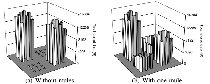
Fig. 12. Distribution of total stored data after one hour
