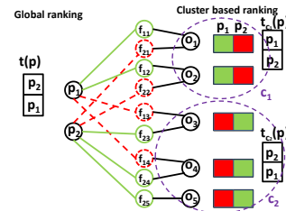
Figure 1: Trustworthiness information propagation should be restrictive
