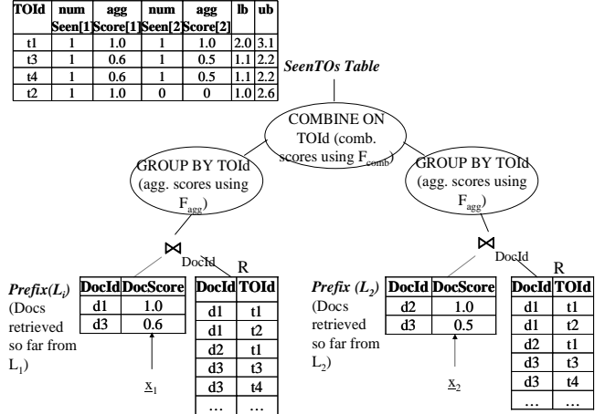
Figure 5: Query Evaluated over the prefixes Prefix(L_i) in each iteration.
