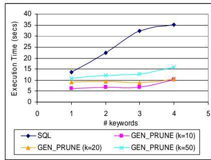
Figure 15: Sensitivity of GEN_PRUNE and SQL approaches to the number of keywords
