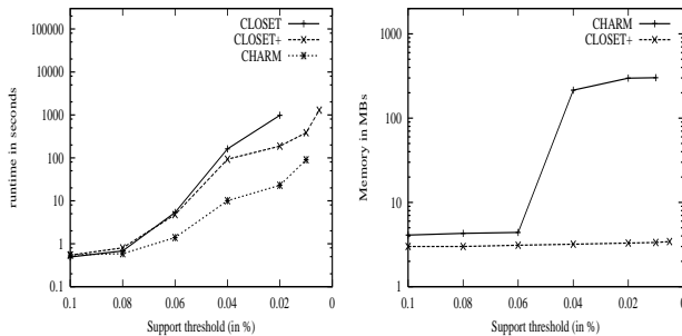
Fig. 14. Runtime performance ( gazelle ).
