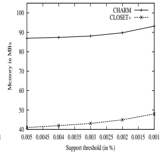
Fig. 19. Memory usage ( big-market ).
