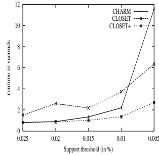
Fig. 16. Runtime performance ( retail-chain ).
