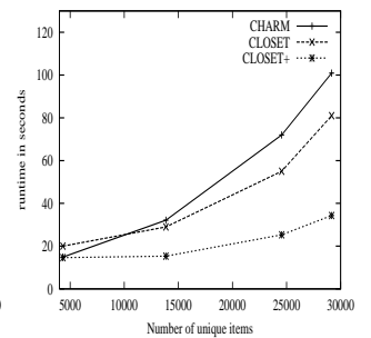
Fig. 21. Scalability test ( T10I4D100kPx ).
