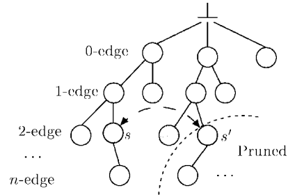
Fig.5. Search space.
