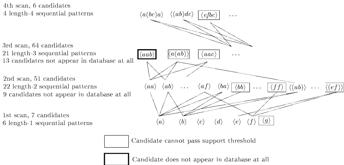
Fig.1. Candidates, candidate generation, and sequential patterns in GSP.
