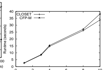
Figure 9. The scalability of runtime on dataset T10I4D100-1000k .
