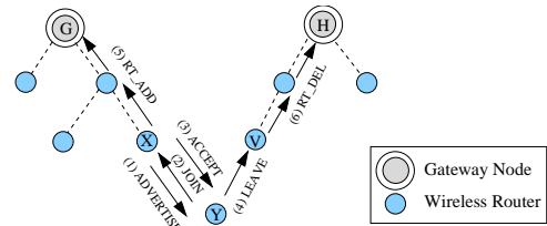
Fig. 2. A distributed route discovery/update protocol used to establish routes between multi-channel WMN nodes and wired gateways.
