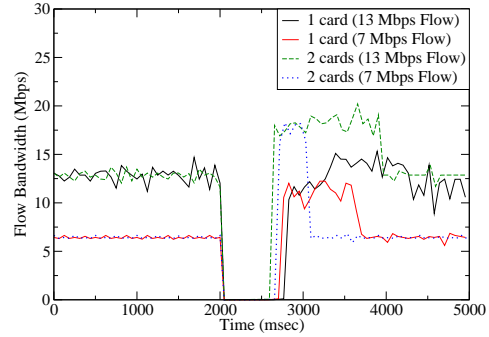
Fig. 17. Failure recovery time for Node 3 in Fig 16, when Node 6 fails. Failure occurs at time 2000 msec, and network recovers within 700 msec.
