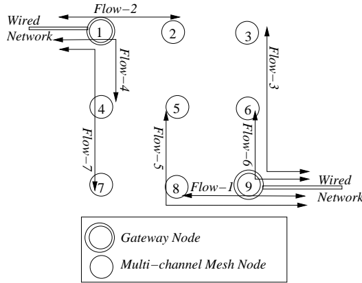
Fig. 16. Physical topology of the 9-node Hyacinth prototype. Each node is equipped with 2 802.11a PCI NICs whose channels are tuned dynamically by the channel/route daemon. Two of the nodes 1 and 9 are connected to the department network providing access of departmental computing resources and the Internet.
