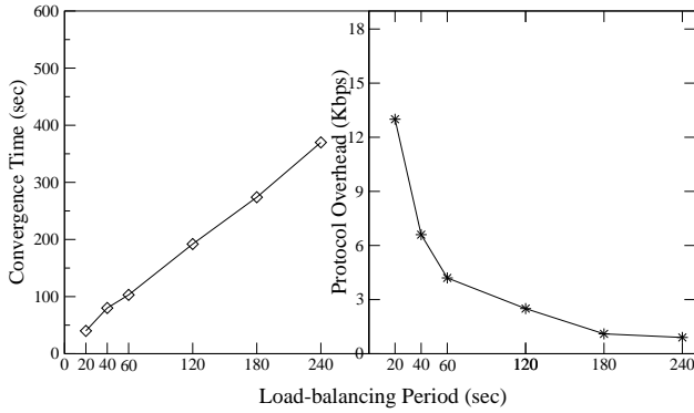
Fig. 15. Impact of load-balancing period on network convergence time against change in traffic load, and the corresponding bandwidth overhead. The network typically converges in less than 2 load-balancing periods, because the load-balancing periods for different nodes are de-synchronized. The bandwidth overhead due to load balancing actions is relatively low even for a small load-balancing period of 20 seconds, and reduces logarithmically with increasing load-balancing period.
