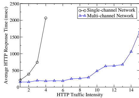
Fig. 7. Web browsing (HTTP) response time as seen by users on a 64-node WMN. The multi-channel mesh network architecture can drastically reduce the HTTP response time, as well as increase the number of users a network can support.
