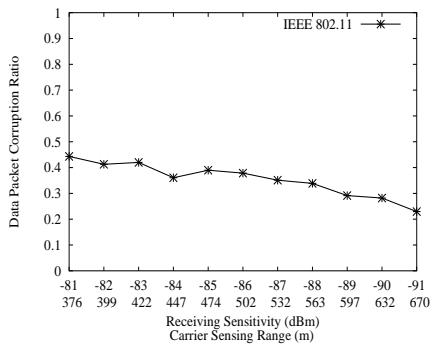
Fig. 13. Pkt corruption ratio vs. CS range. Fig. 14. Agg. throughput vs. CS range. Fig. 15. Data pkt delivery ratio vs. CS range.
