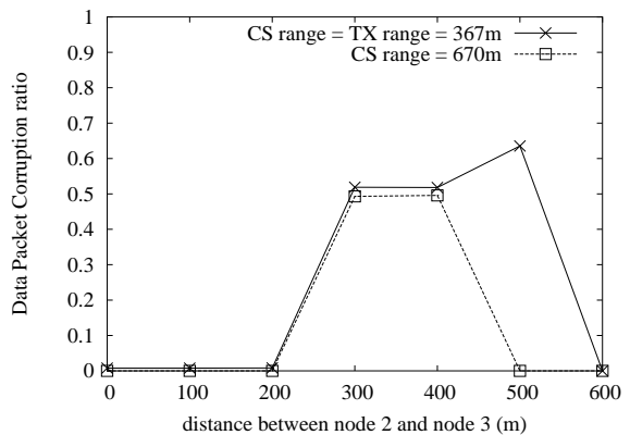
Fig. 7. Pkt corruption ratio vs. distance between node2 and node3.
