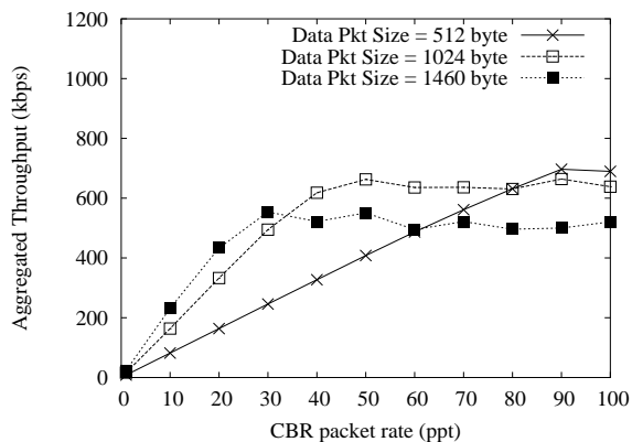
Fig. 8. Aggregated throughput vs. CBR packet rate and size.
