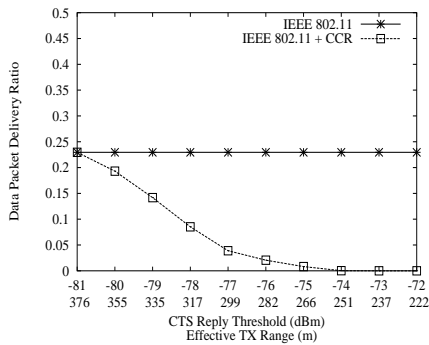
Fig. 16. Data Packet corruption ratio vs. CTS-Reply-Threshold.
