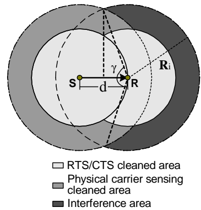
Fig. 12. Upper bound of the beam width
