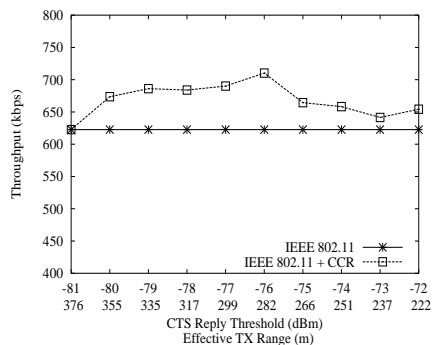
Fig. 17. Agg. throughput vs. CTS-Reply-Threshold.
