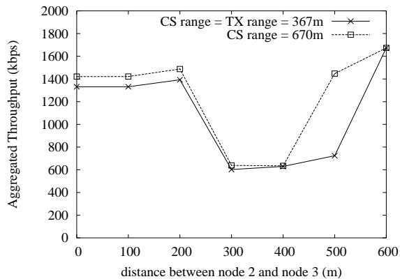
Fig. 6. Agg. throughput vs. distance between node2 and node3.
