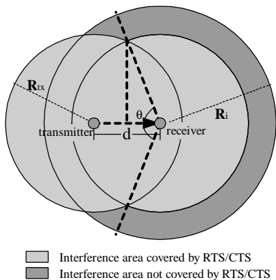
Fig. 1. Effectiveness of RTS/CTS handshake when d is larger than T_{SNR}^{-\frac{1}{k}} * R_{tx} and smaller than R_{tx} .
