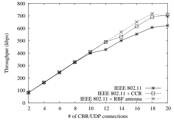
Fig. 20. Aggregated throughput vs. # of CBR pairs.
