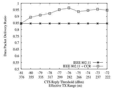
Fig. 18. Data pkt delivery ratio vs. CTS-Reply-Threshold.
