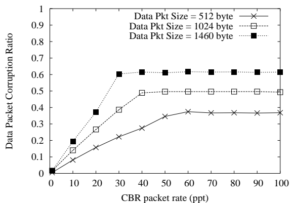
Fig. 9. Packet corruption ratio vs. CBR packet rate and size.
