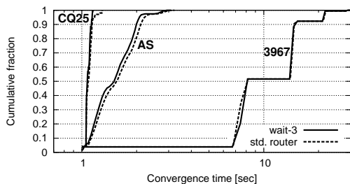
Figure 8: Network-wide simulations, per-router convergence delay distribution.
