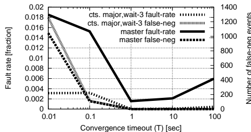
Figure 6: Effect of convergence time threshold.
