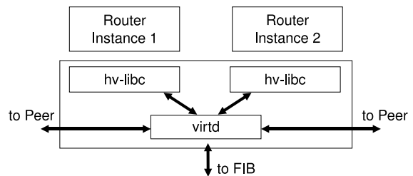
Figure 2: Implementation architecture.
