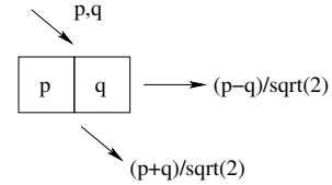
Figure 5: The algorithm A_\ell
